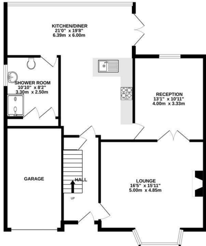
GROUND FLOOR 975 sq.ft. (90.6 sq.m.) approx.
